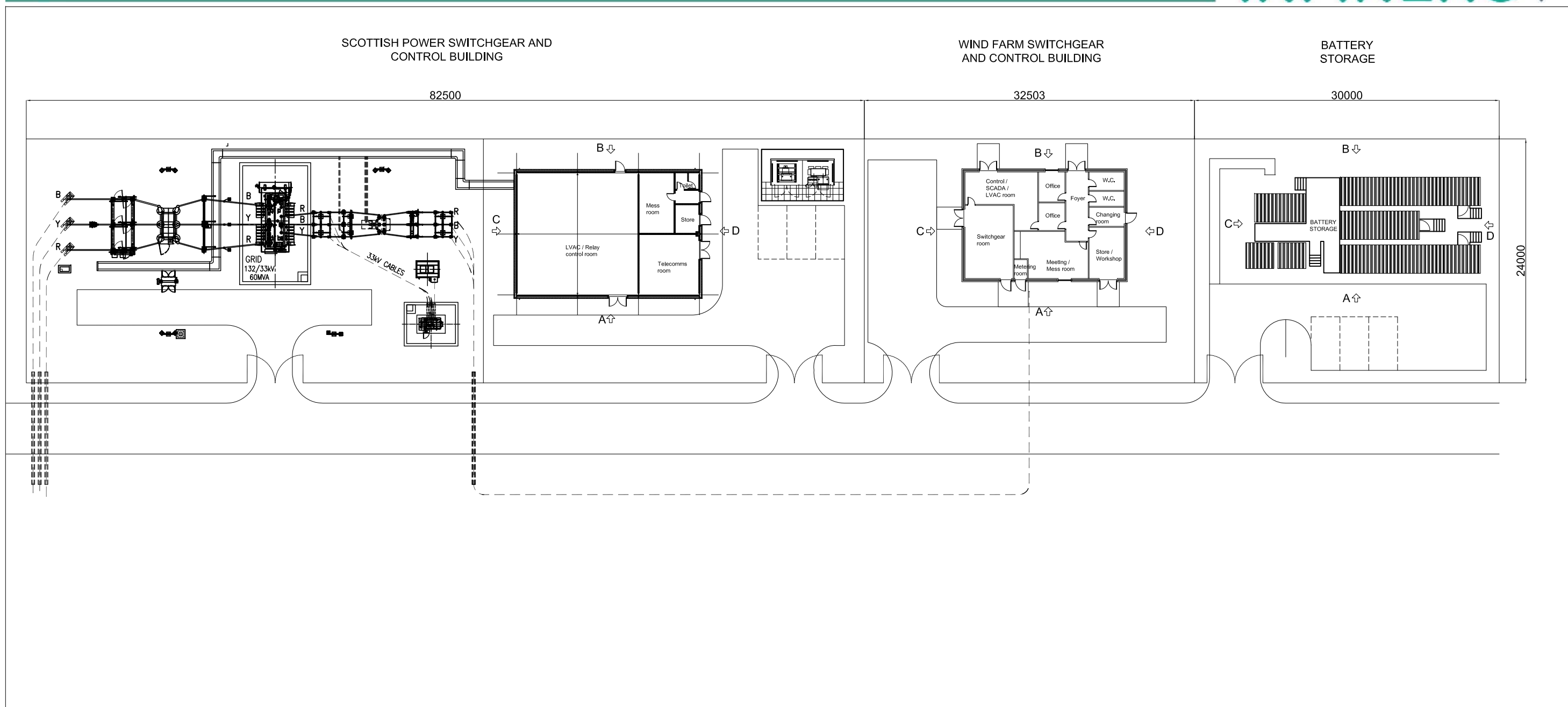
Figure 4.10: Indicative Substation Compound Layout
