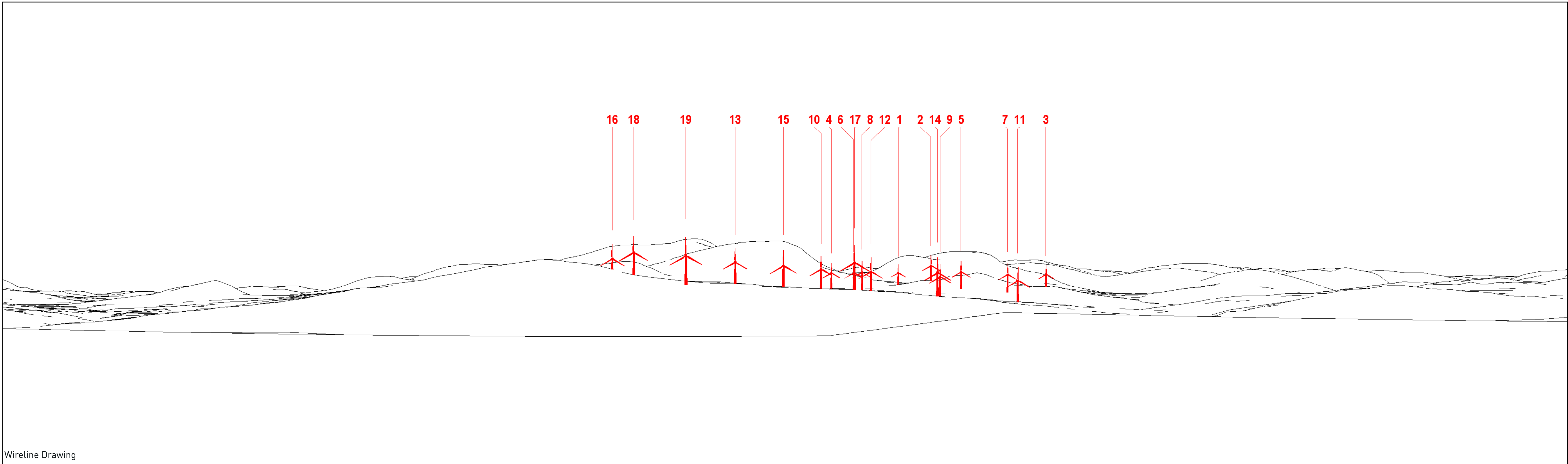
Figure 11.10 Wireframe visualisation from Culmark Hill Cairn SHEPHERDS' RIG WIND FARM
