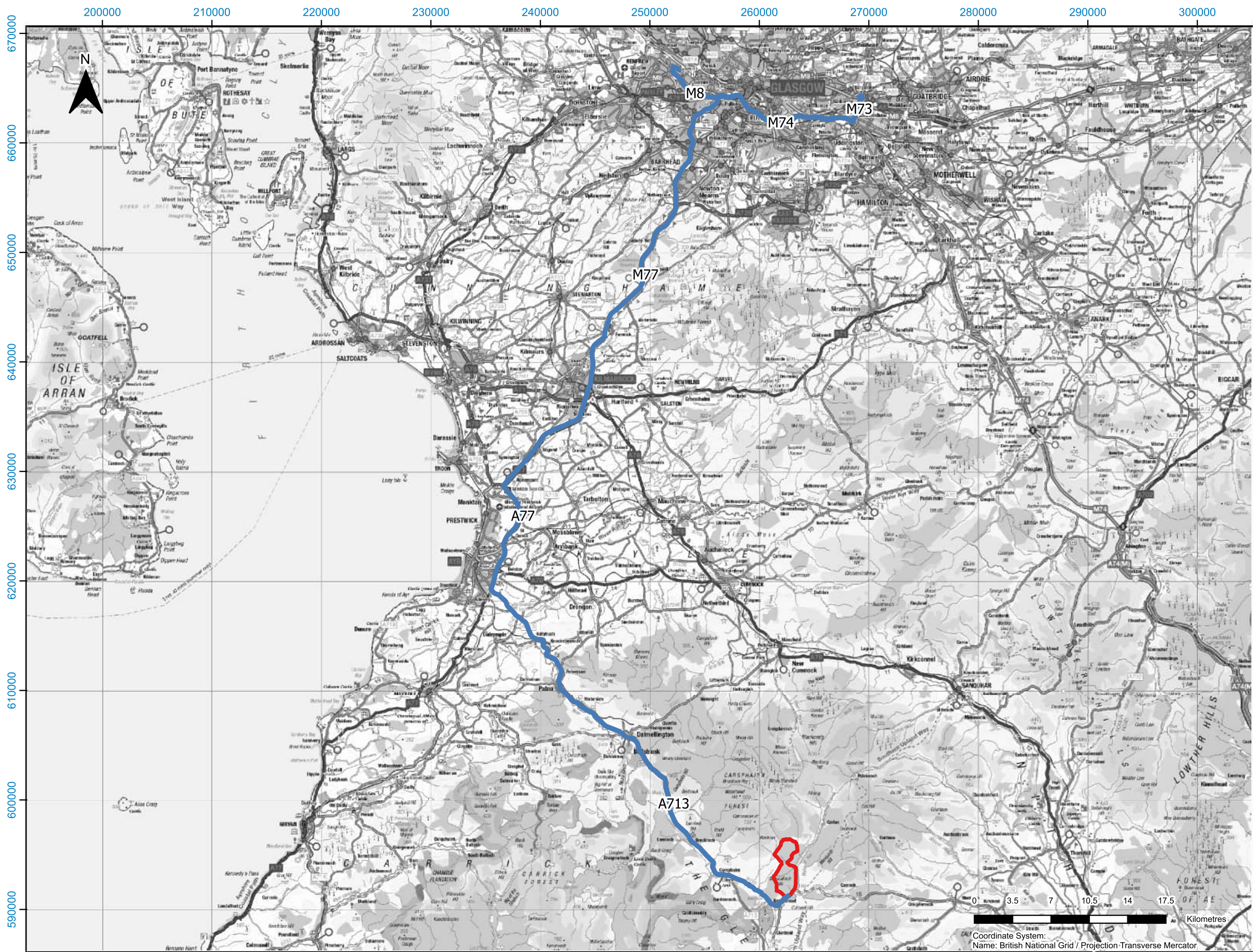
Figure 15.4: Abnormal Indivisible Load Delivery Route
