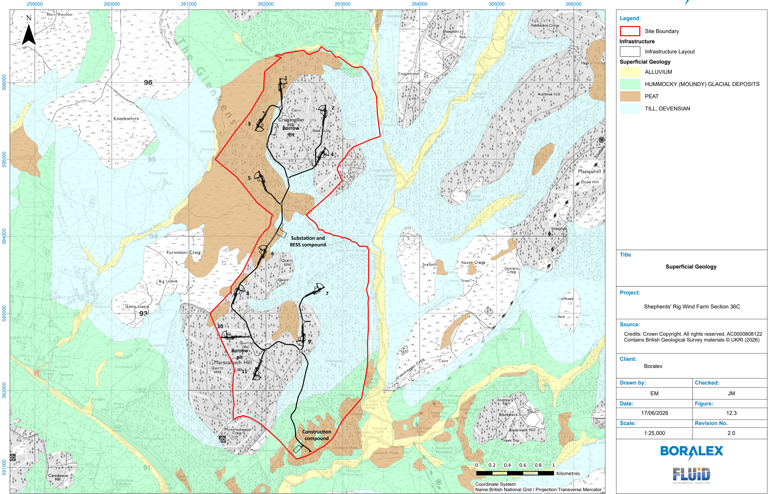
Figure 12.3: Superficial Geology
