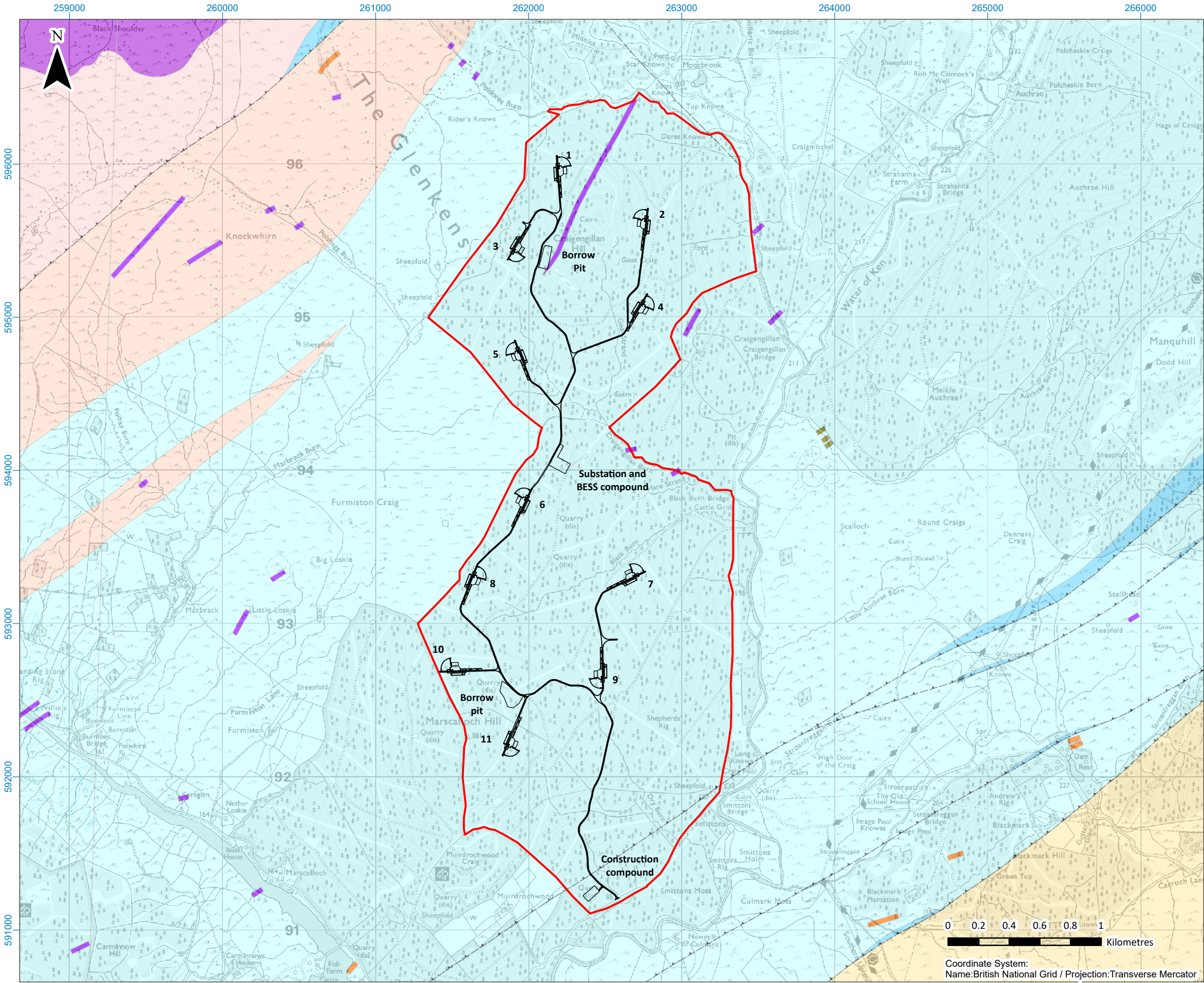
Figure 12.4: Bedrock Geology
