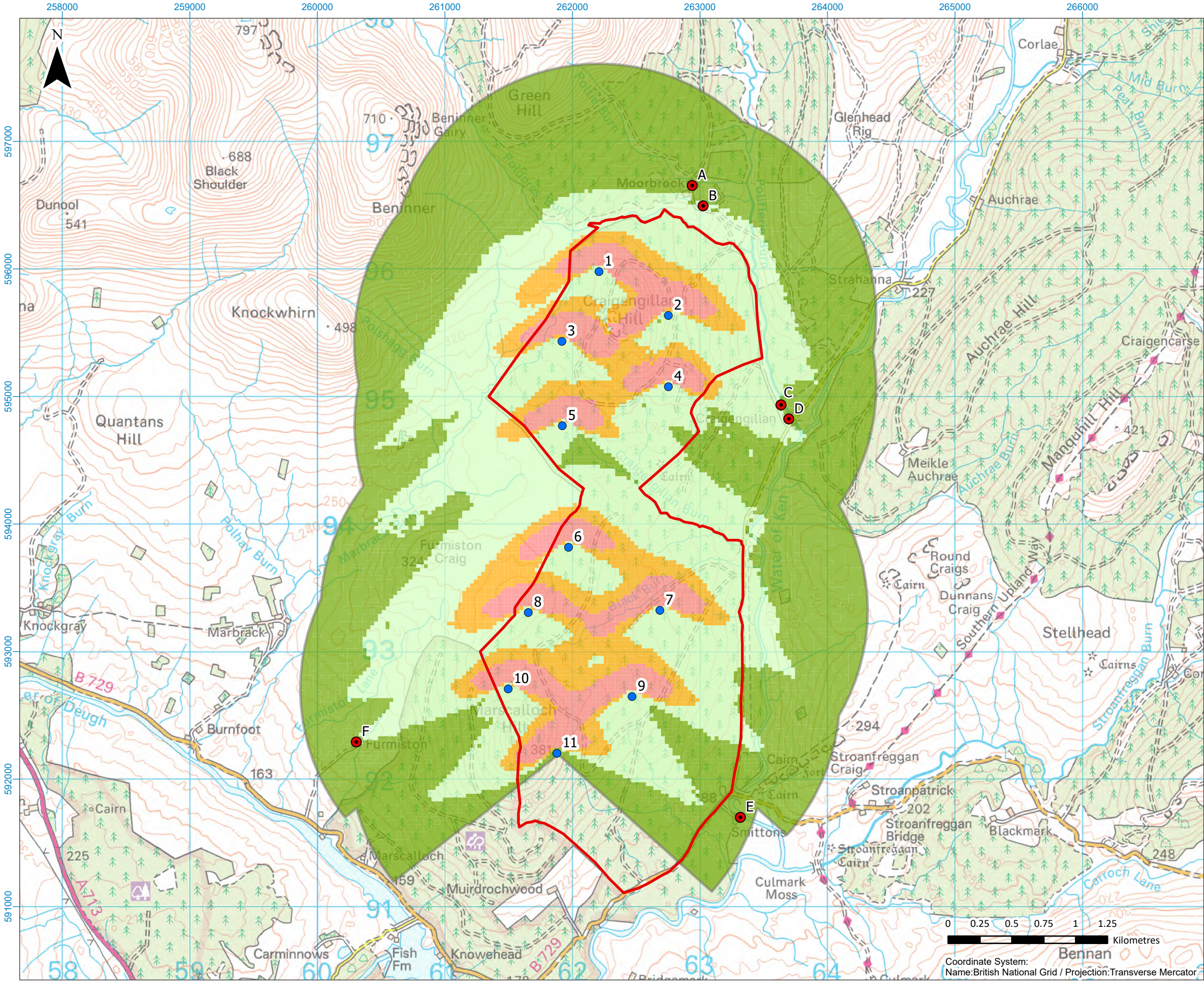
Figure 17.2: Shadow Flicker Results (Realistic Scenario)
