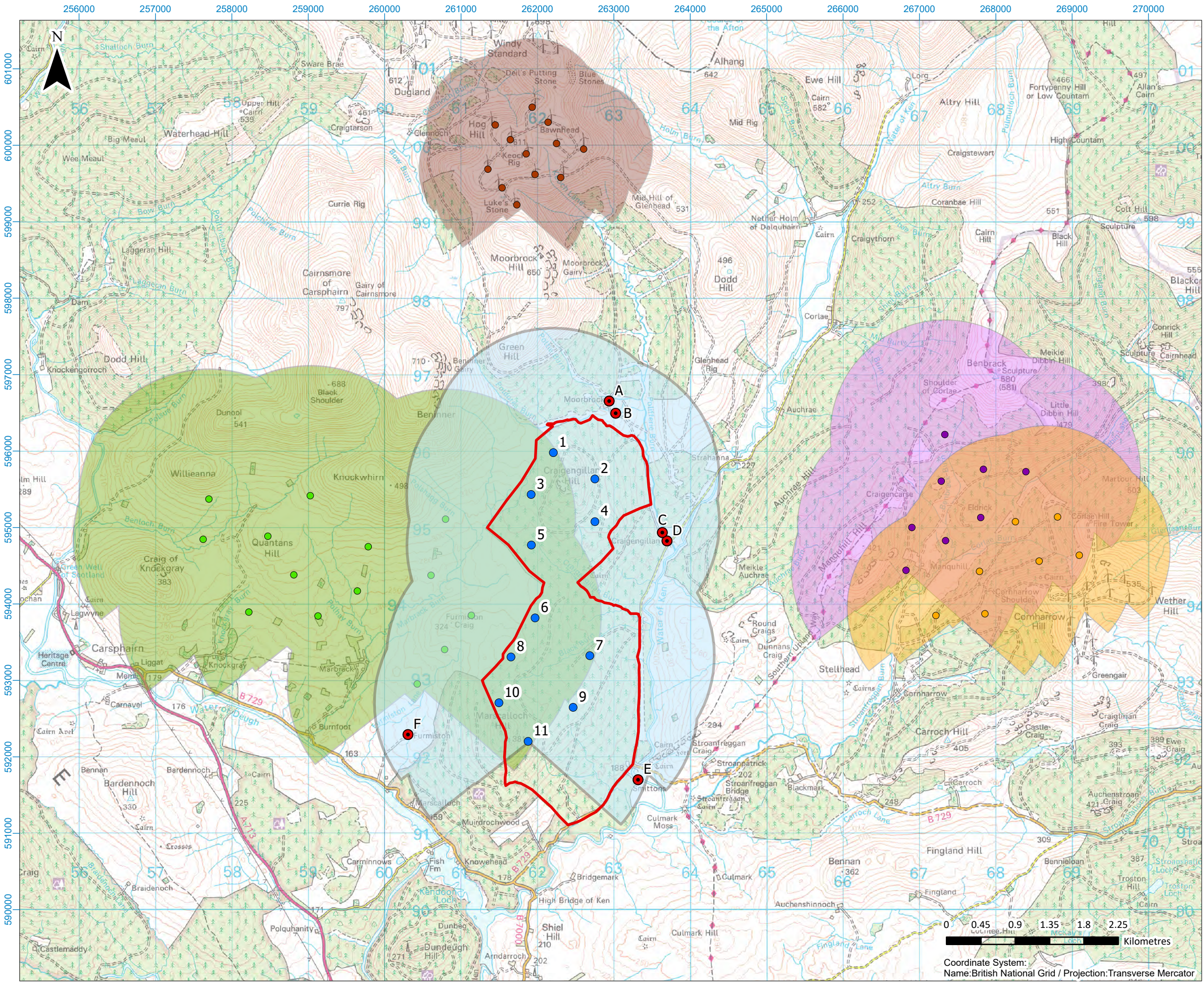
Figure 17.3: Cumulative Shadow Flicker Study Area
