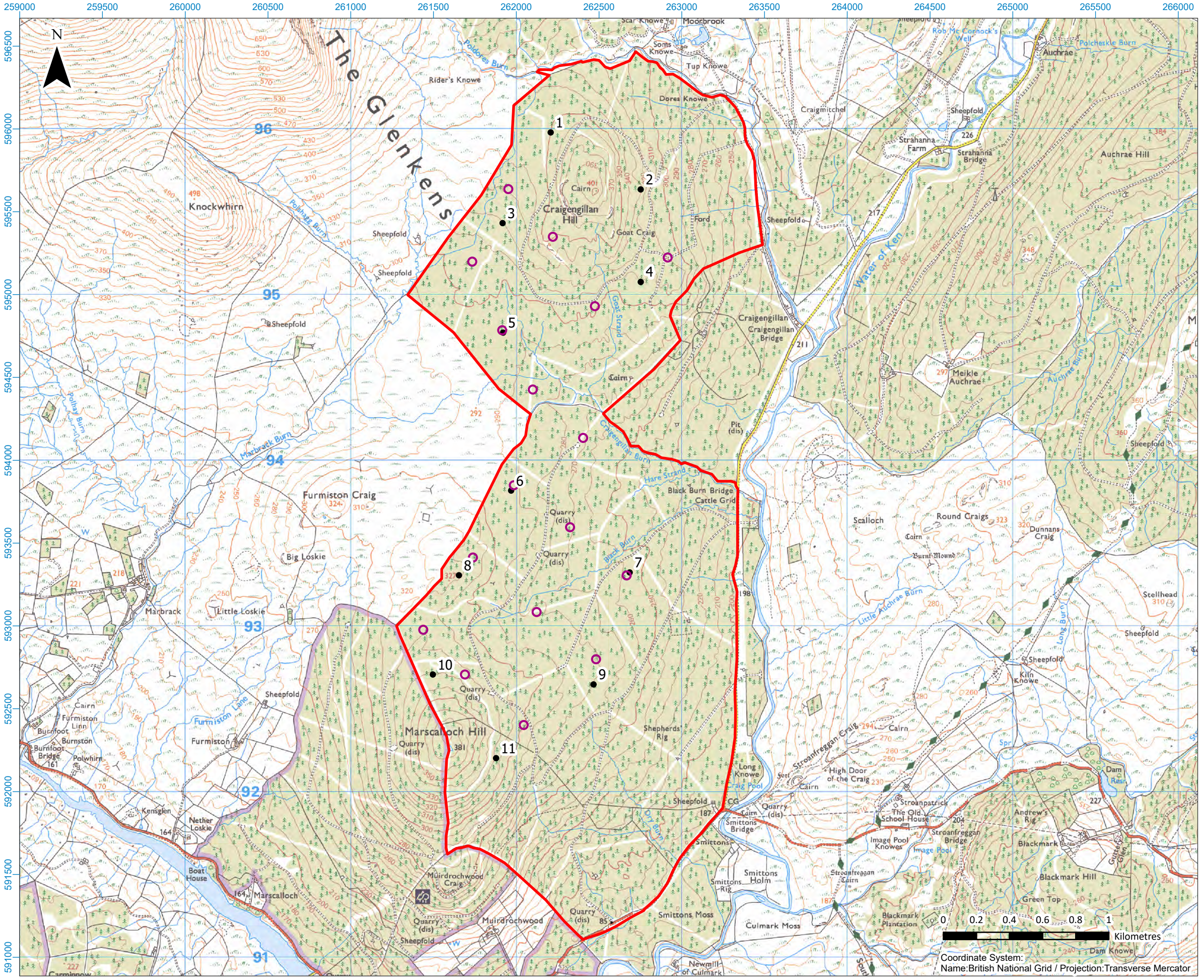
Figure 4.2: Varied and Consented Turbine Locations
