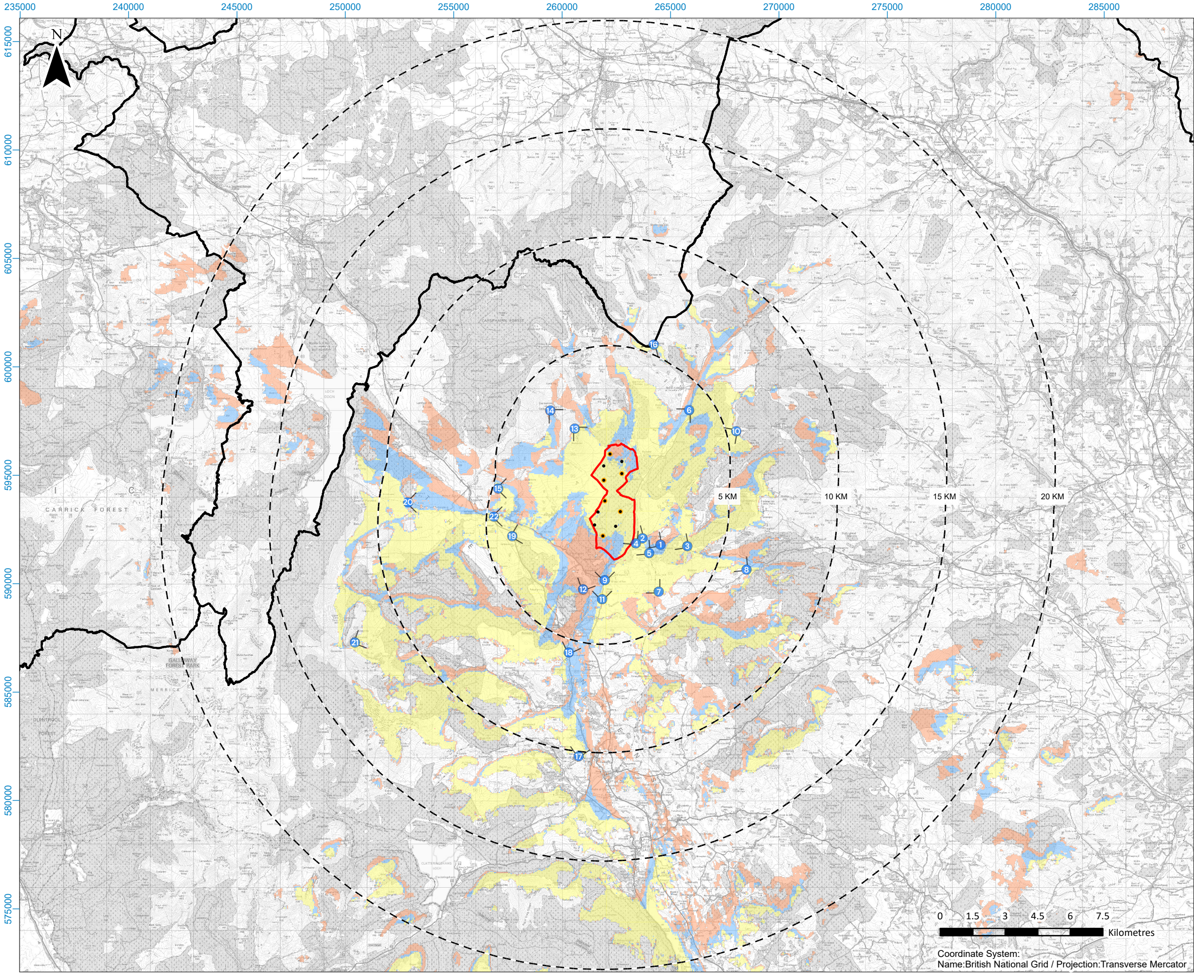
Figure 8.10: Proposed Varied Development Lit Turbine ZTV to 20 km with Viewpoints
