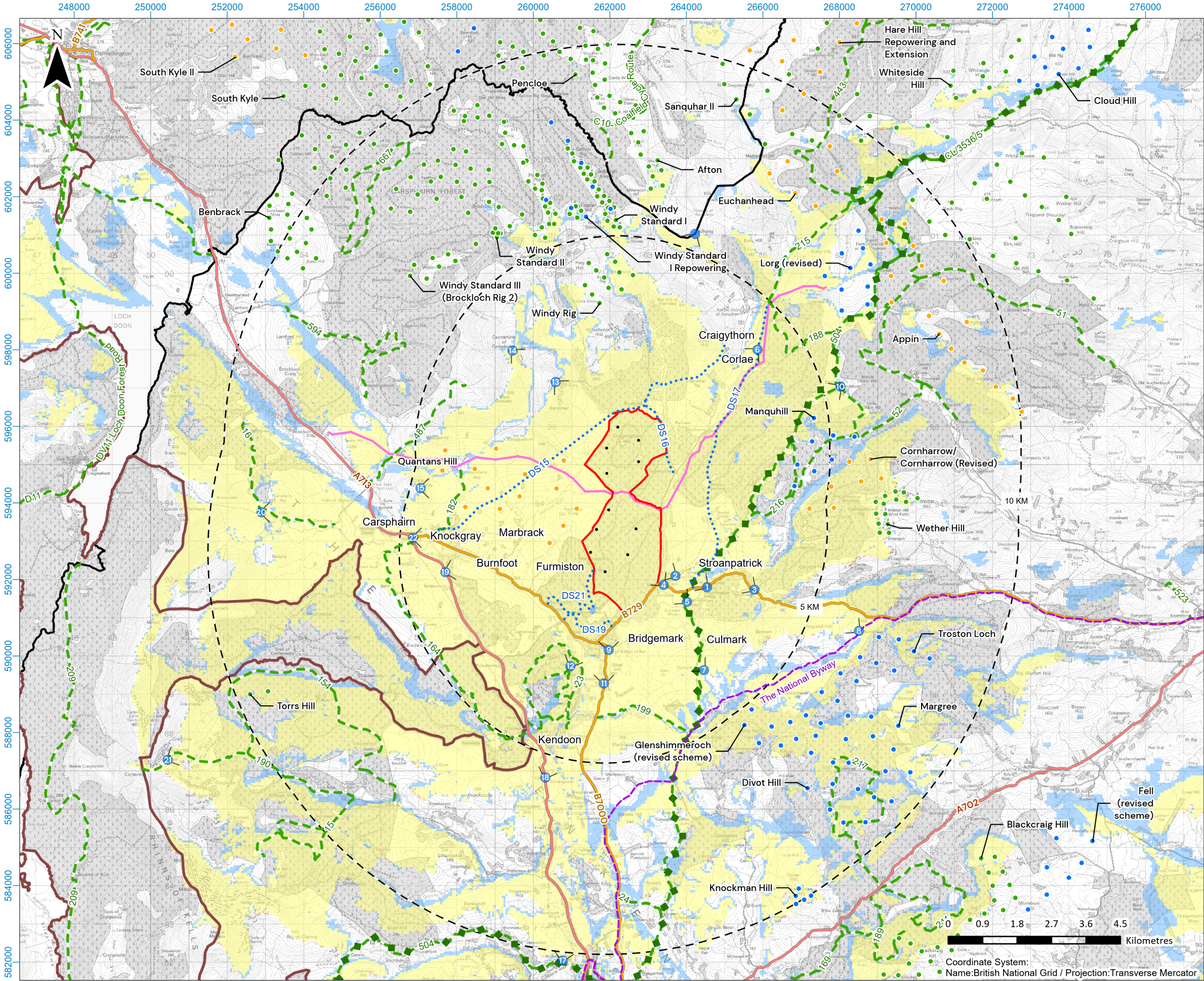
Figure 8.19 Principal Visual Receptors to 10 km with Comparative Blade Tip ZTV and Viewpoints
