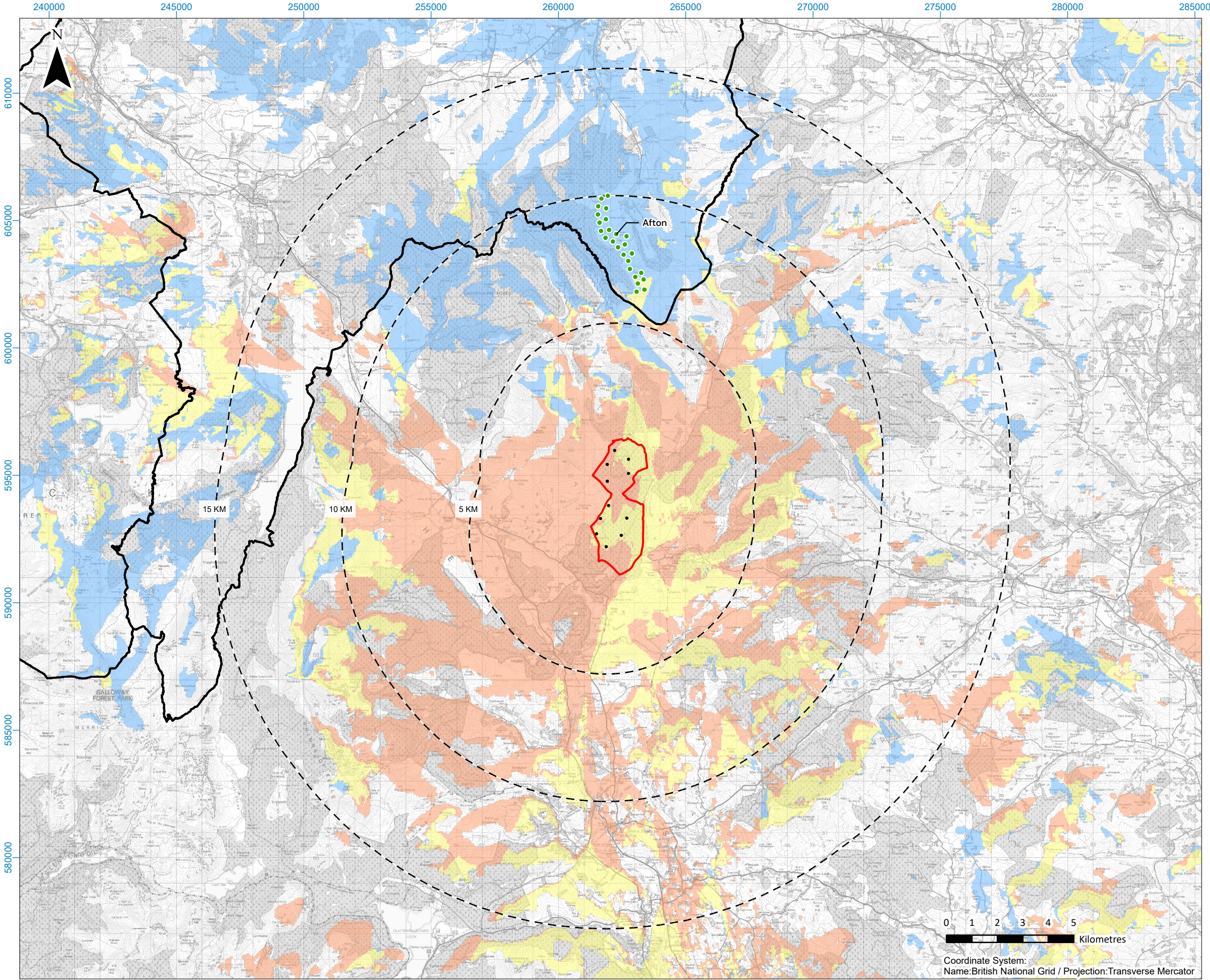
Figure 8.21 - Cumulative ZTV with Operational/Under Construction Afton Wind Farm
