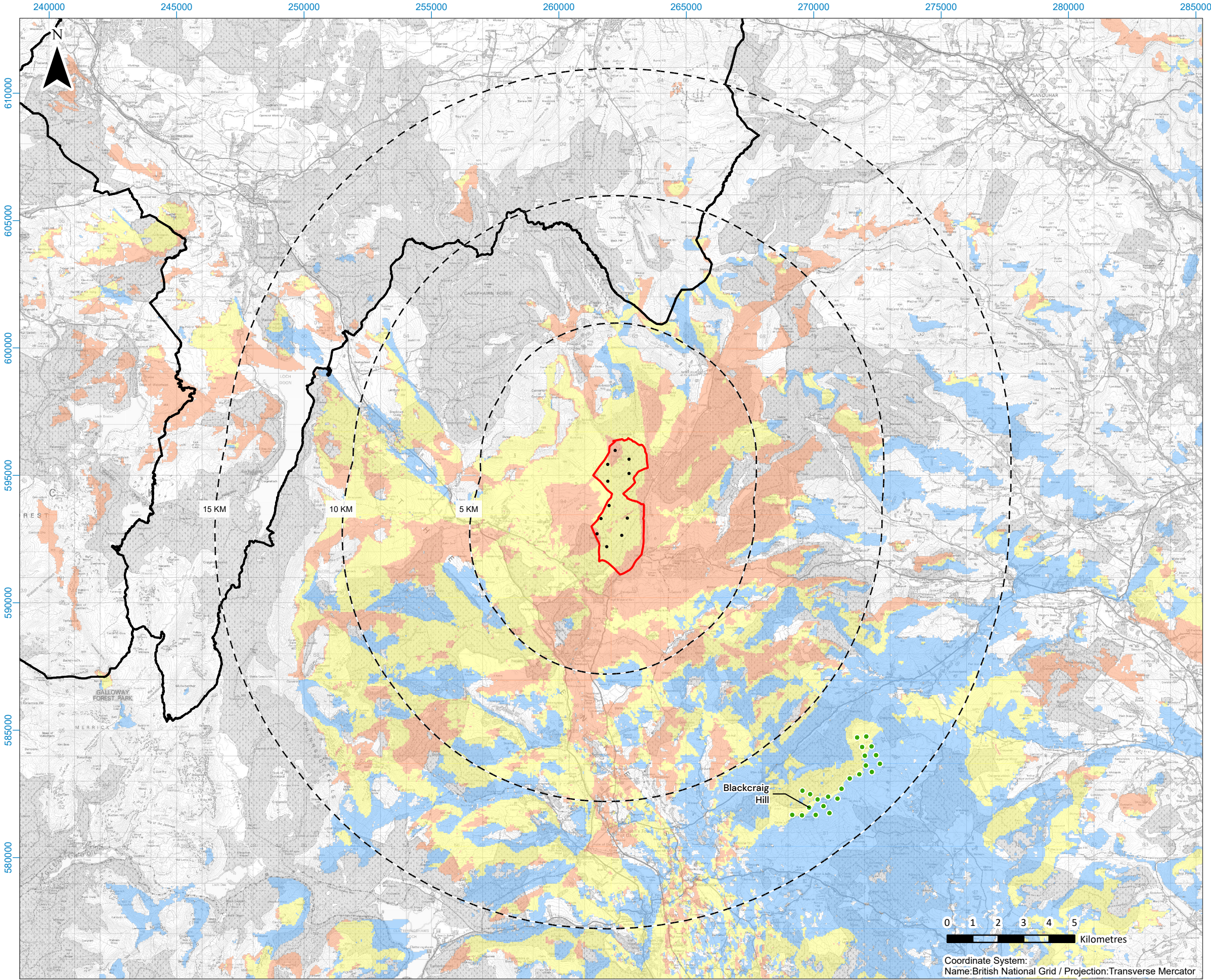
Figure 8.23 - Cumulative ZTV with Operational/Under Construction Blackcraig Hill wind farm
