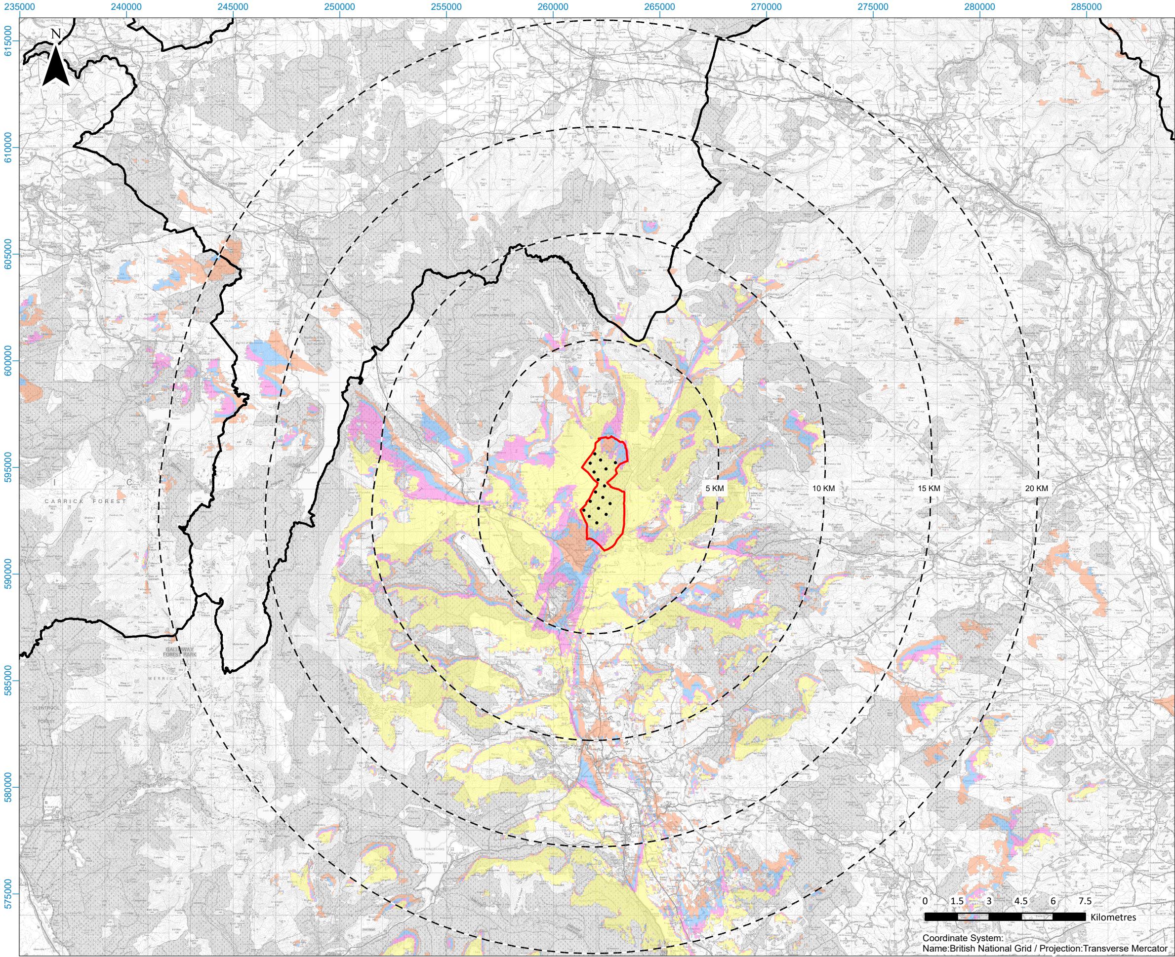
Figure 8.3: Consented Development Blade Tip ZTV to 20 km
