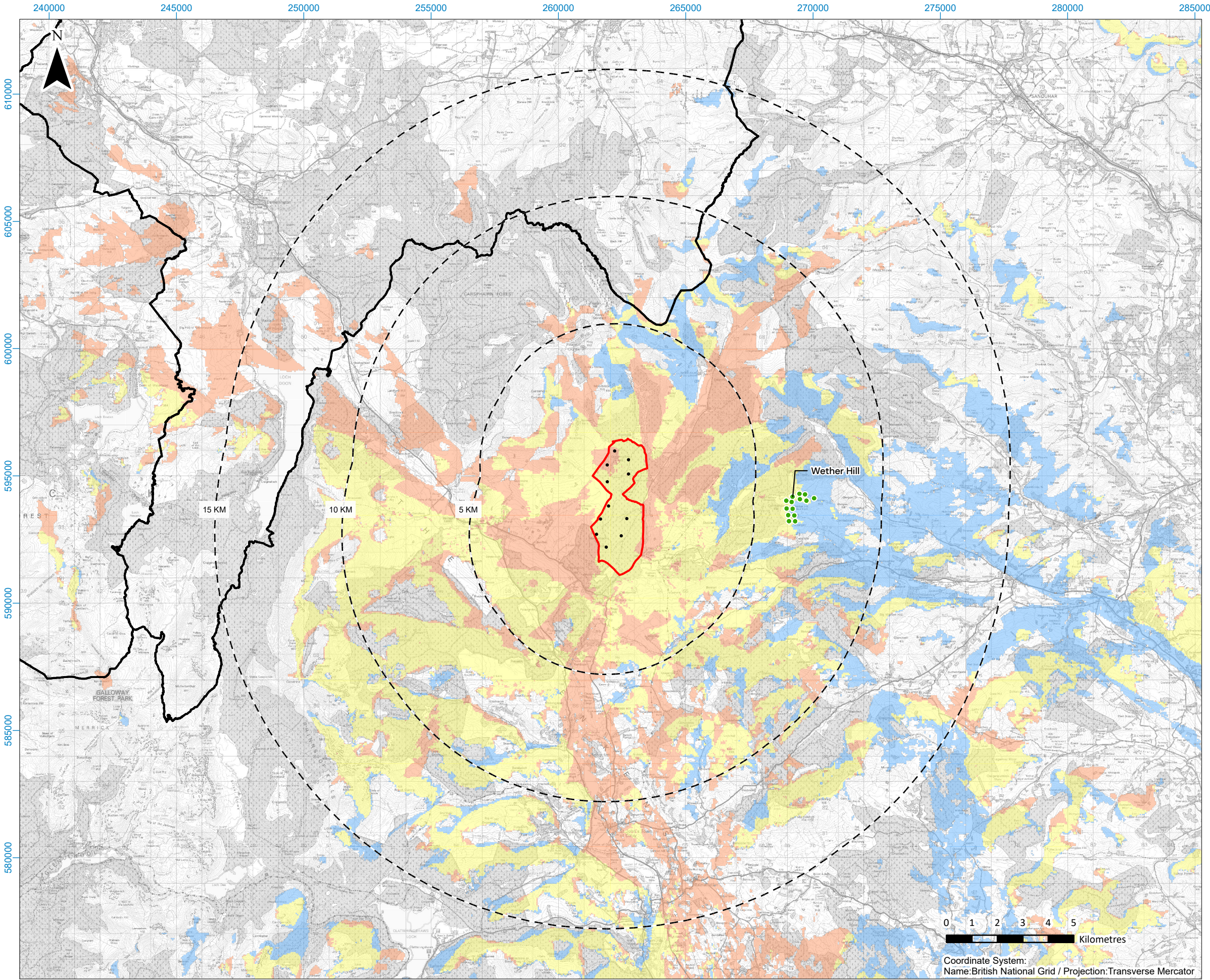
Figure 8.30 - Cumulative ZTV with Operational/Under Construction Wether Hill wind farm
