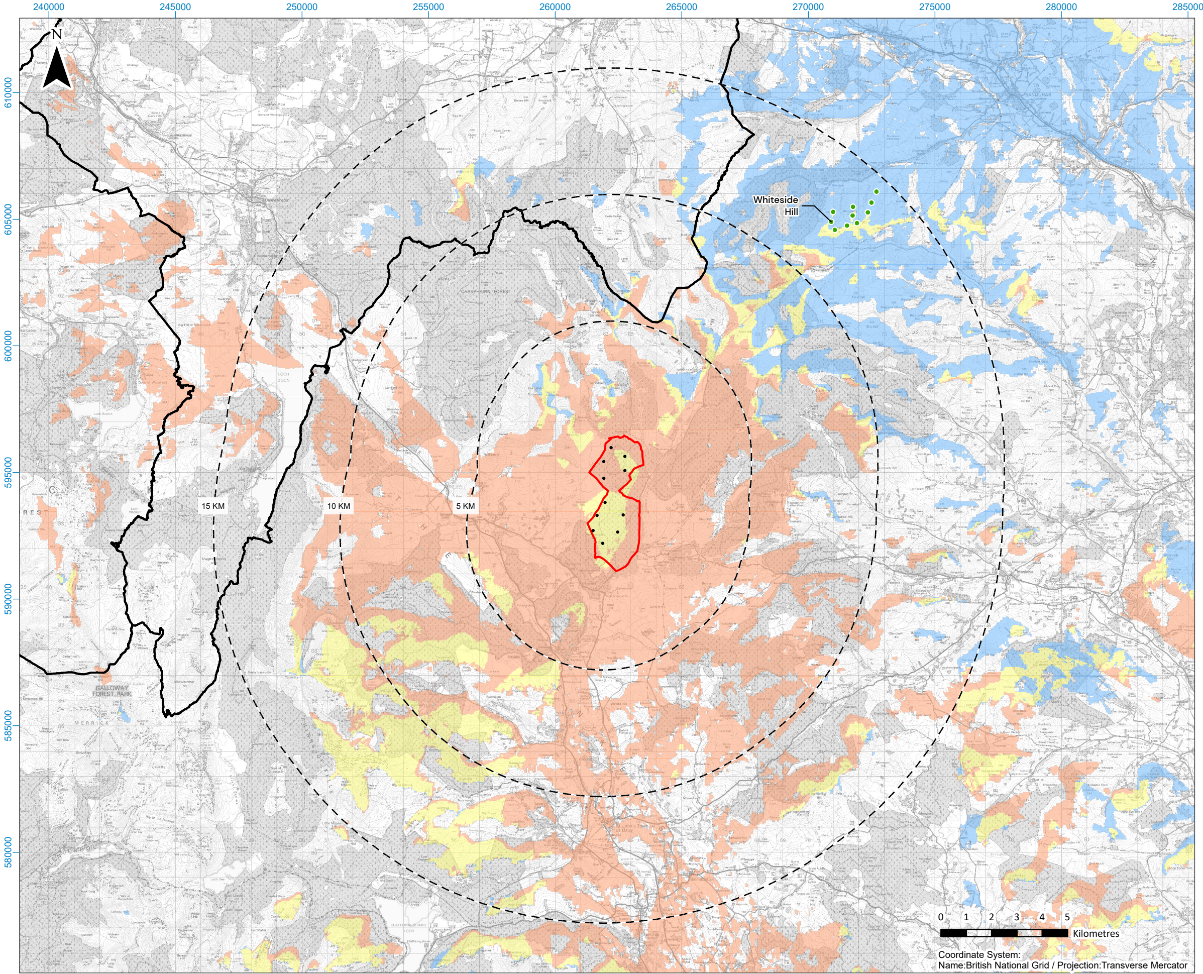
Figure 8.31 - Cumulative ZTV with Operational/Under Construction Whiteside Hill wind farm
