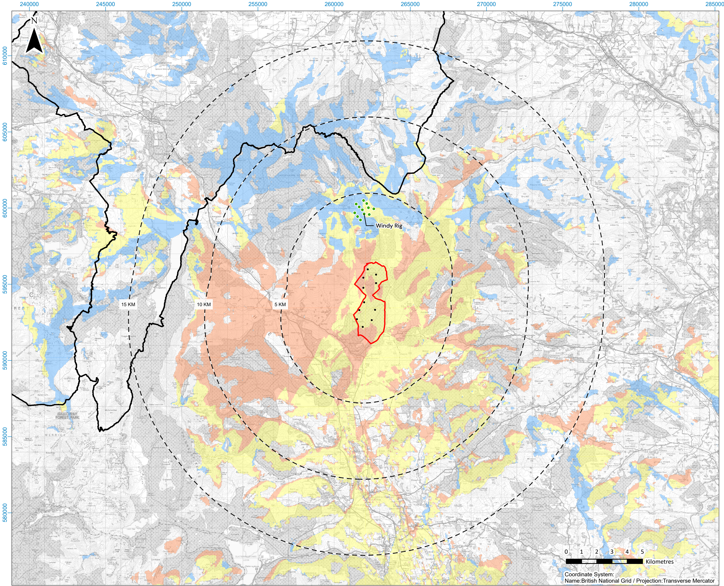
Figure 8.32 - Cumulative ZTV with Operational/Under Construction Windy Rig wind farm
