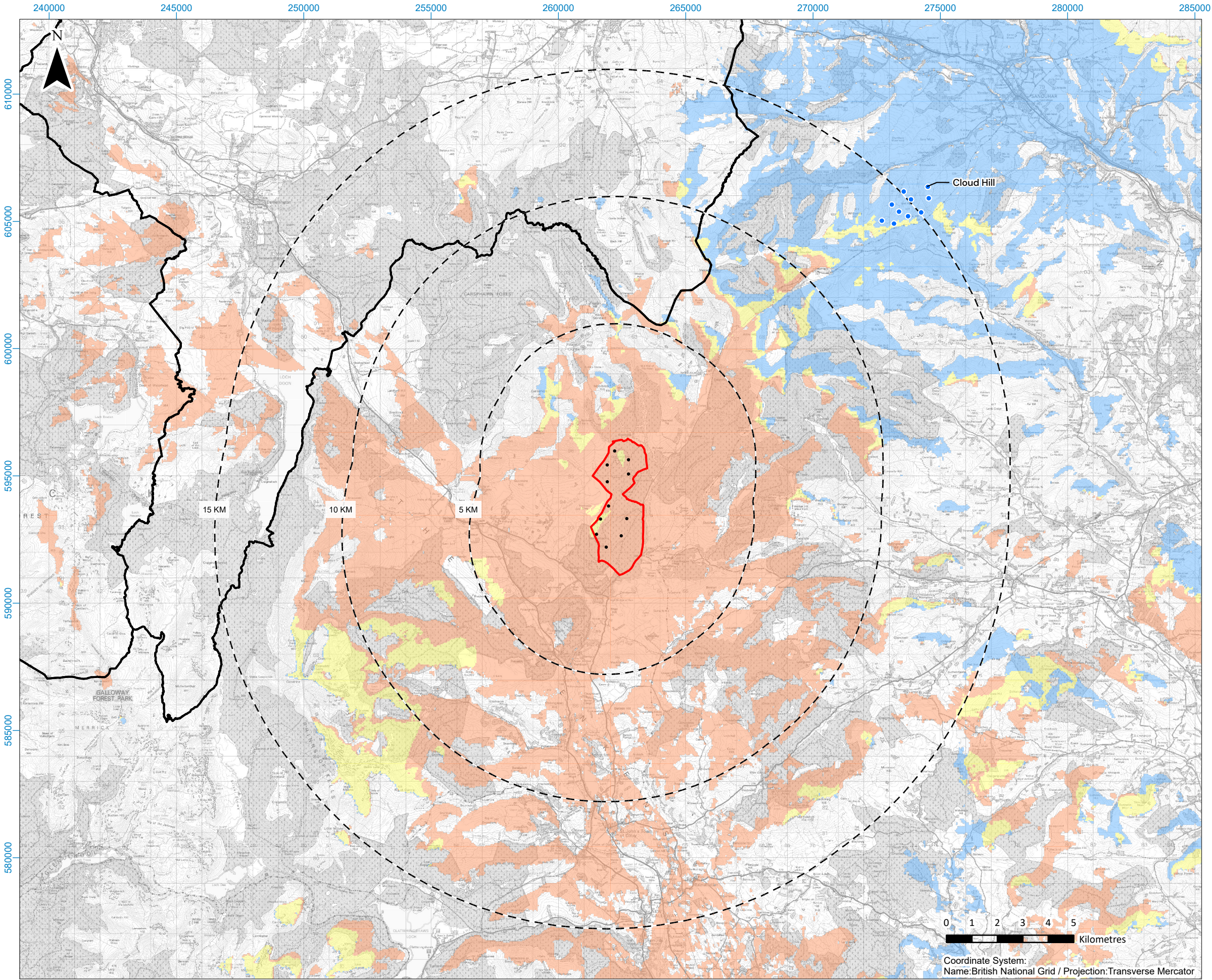
Figure 8.34 - Cumulative ZTV with Consented Cloud Hill wind farm
