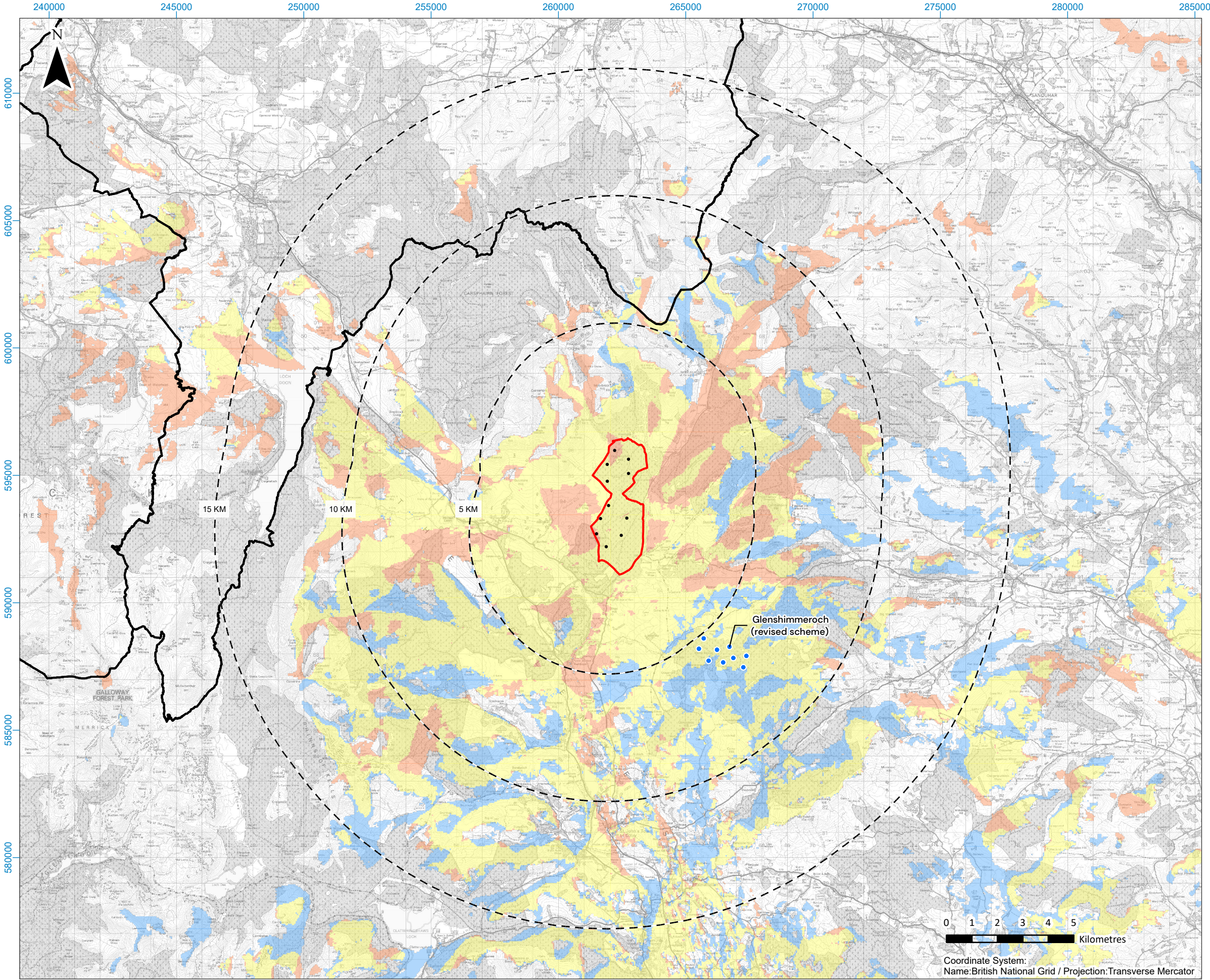
Figure 8.39 - Cumulative ZTV with Consented Glenshimmeroch (revised) wind farm
