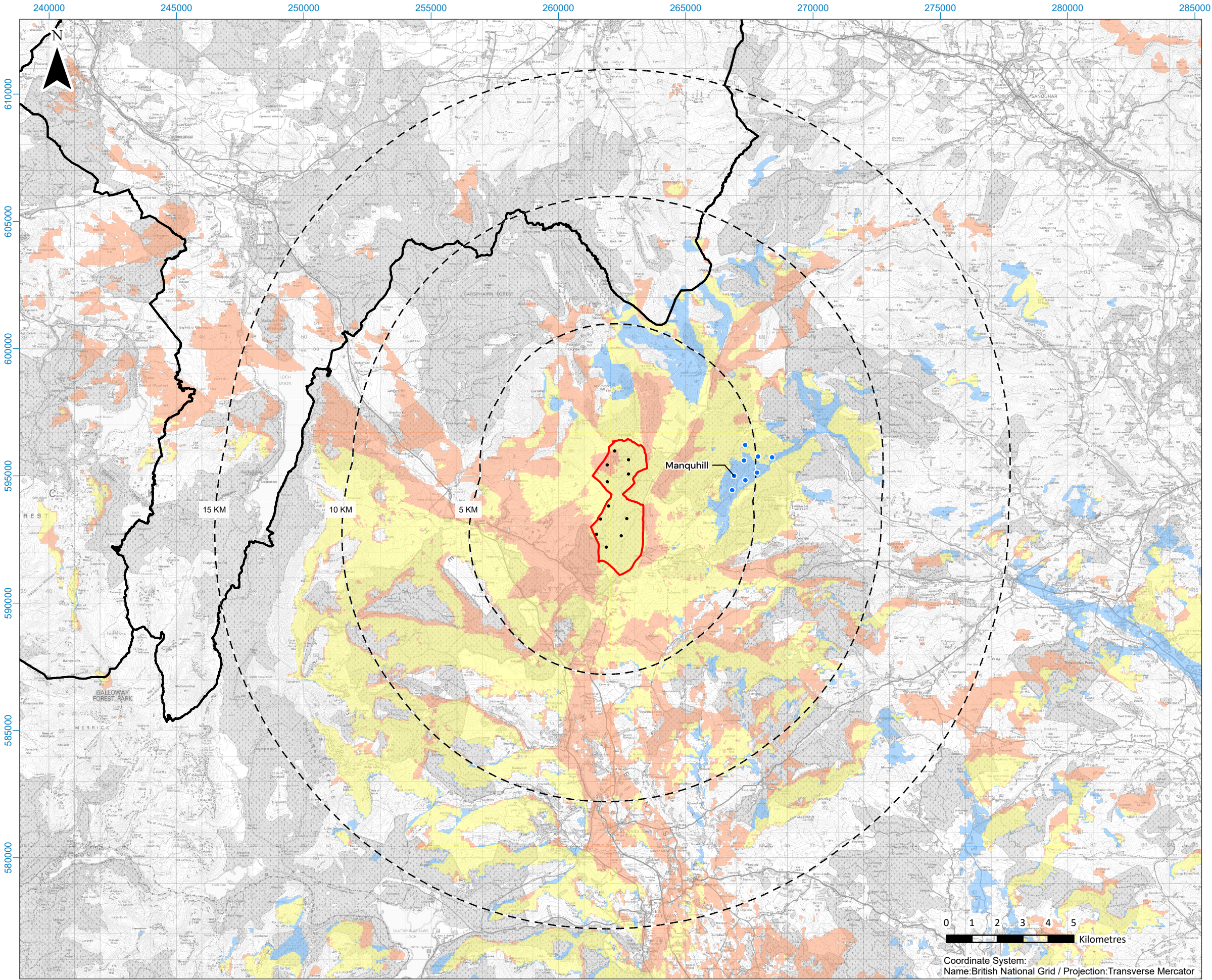
Figure 8.42 - Cumulative ZTV with Consented Manquhill wind farm
