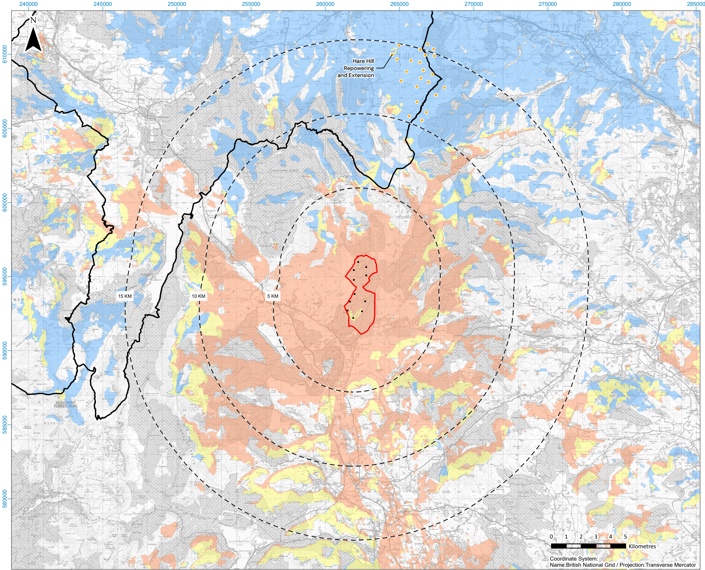
Figure 8.49 - Cumulative ZTV with In Planning Hare Hill Repowering wind farm and Extension
