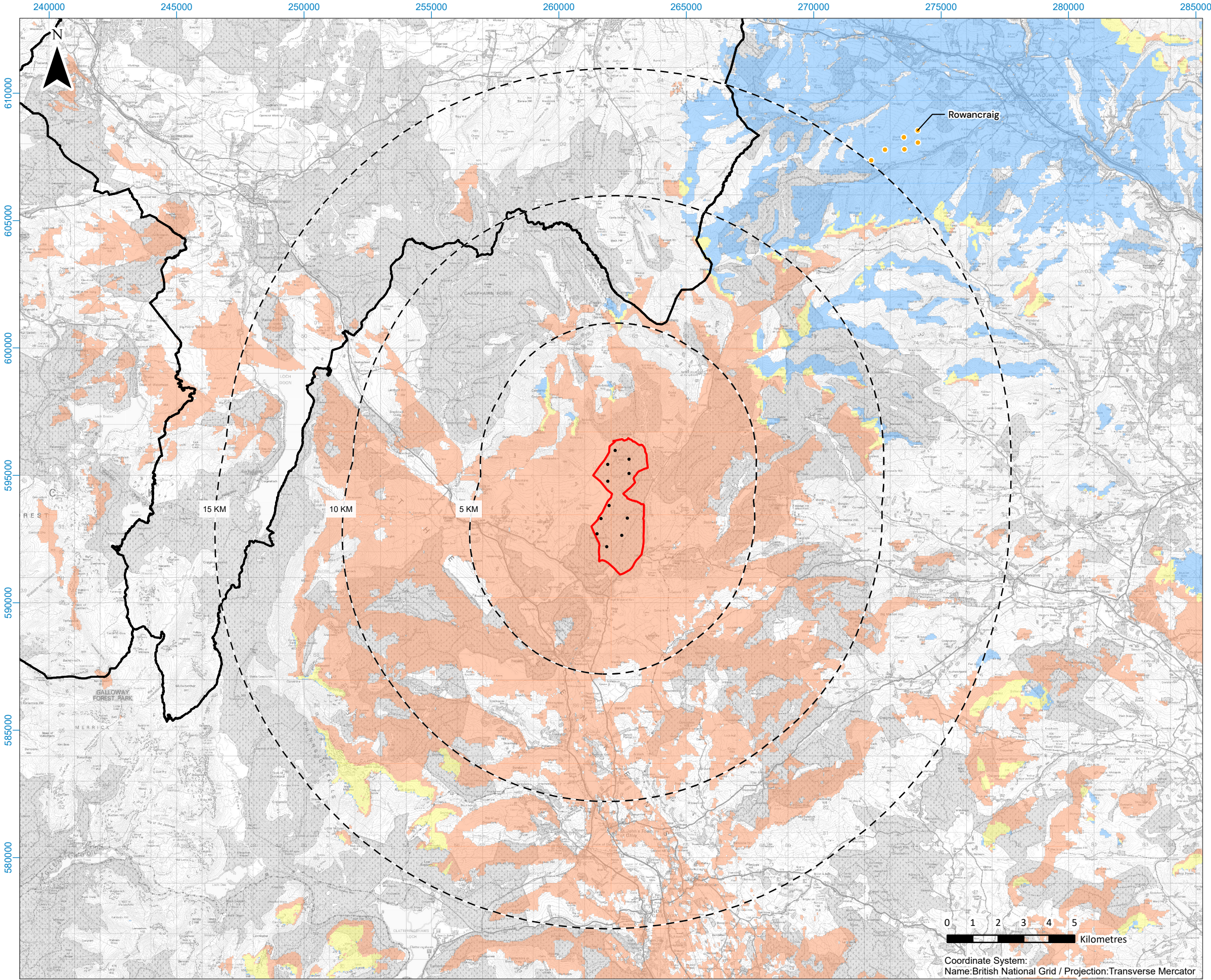
Figure 8.52 - Cumulative ZTV with In Planning Rowancraig wind farm
