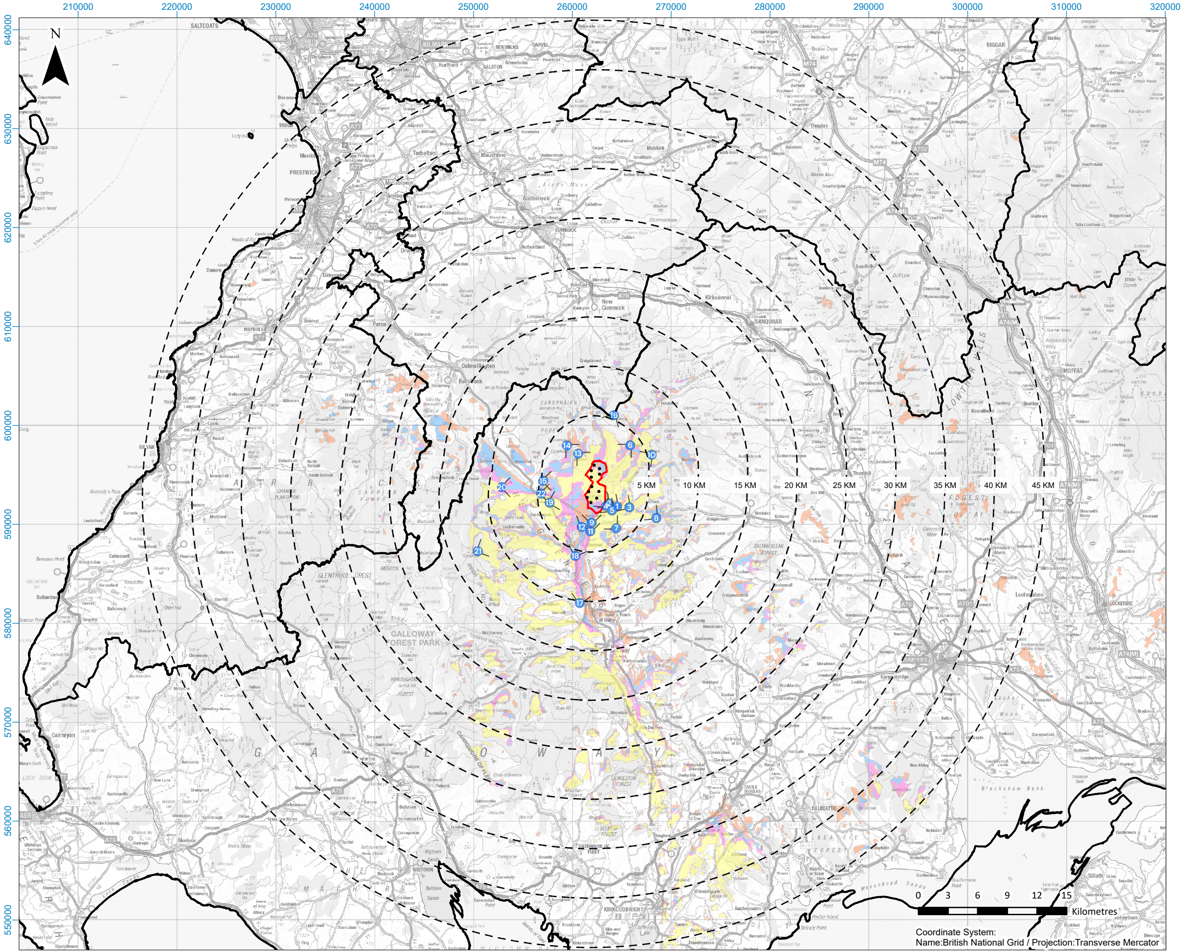
Figure 8.7: Proposed Varied Development Hub Height ZTV to 45 km with Viewpoints
