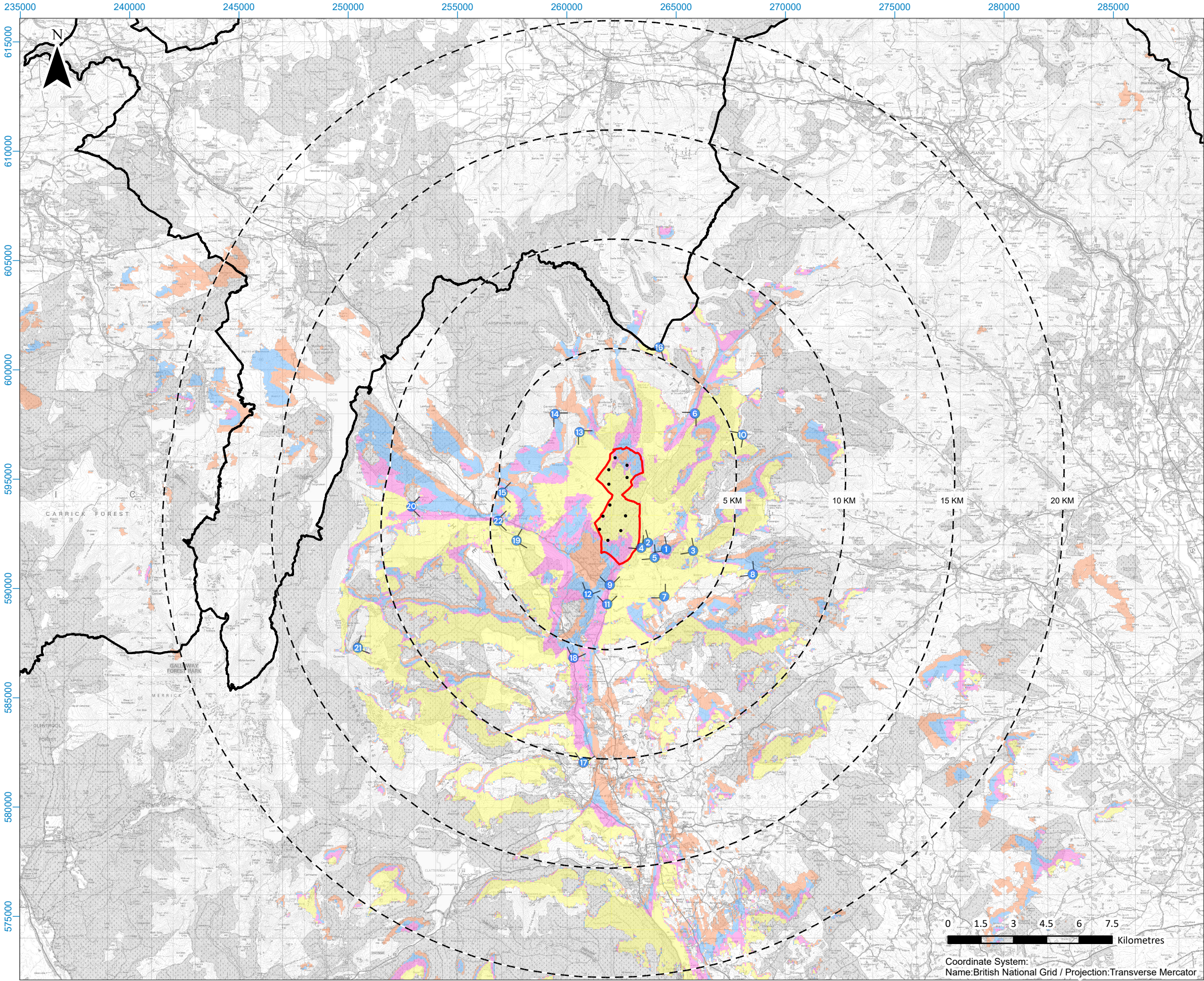
Figure 8.8: Proposed Varied Development Hub Height ZTV to 20 km with Viewpoints
