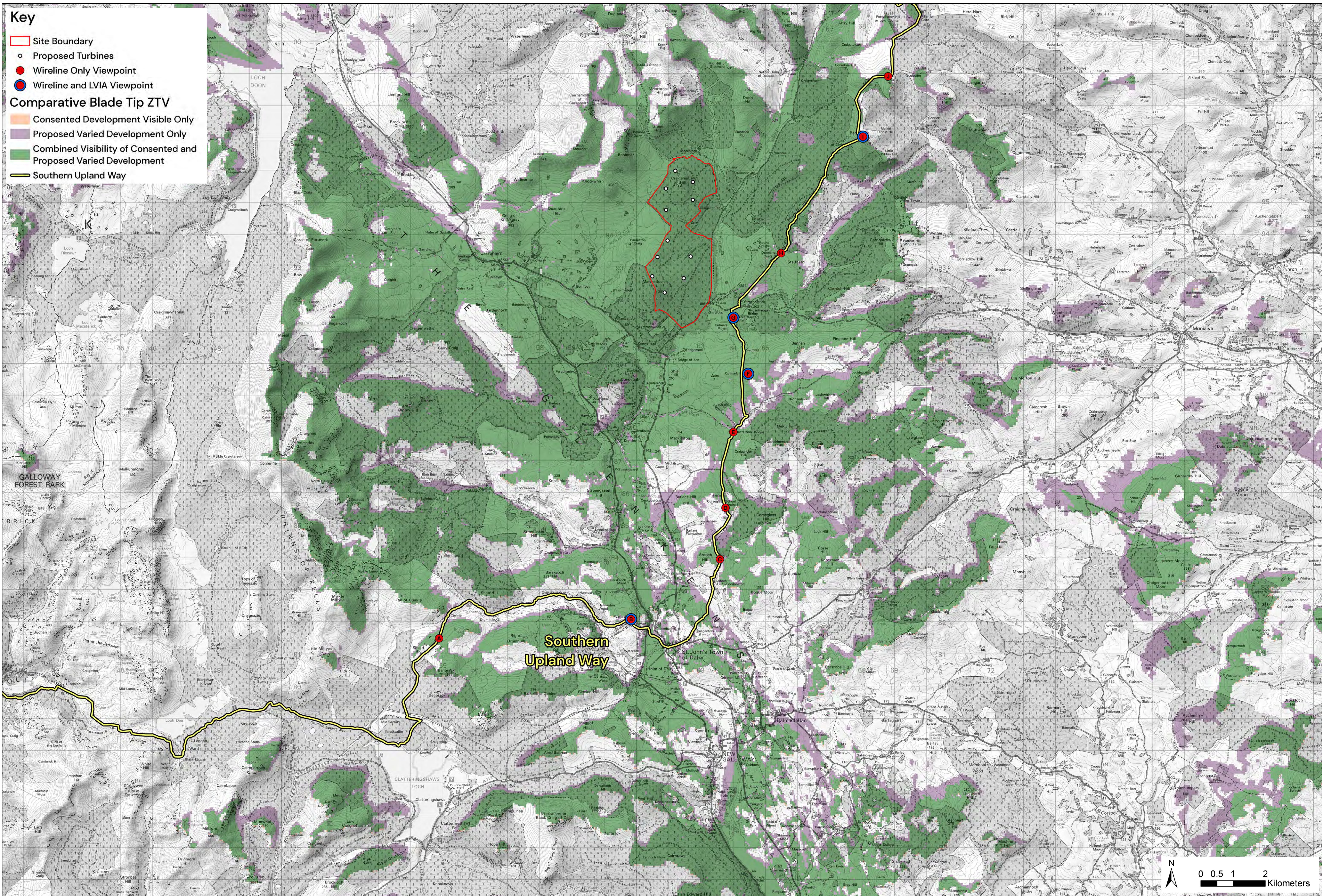
Southern Upland Way Sequential Wireline Viewpoint Location Plan
